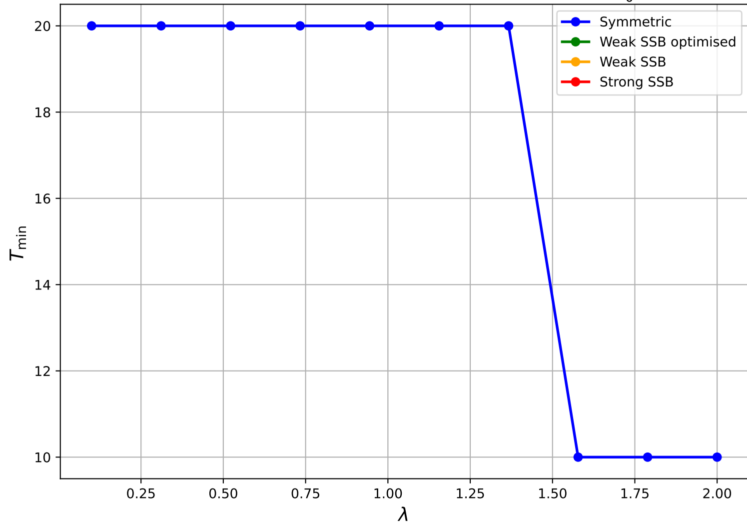
Minimum Adiabatic Time T_{\min} for Fidelity \geq 0.9999 , m_0^2 = 1.0
